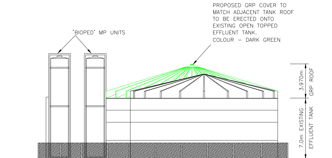
Drawing of effluent plant showing proposed roof for balance tank
