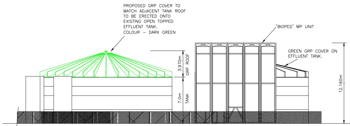
PROPOSED ELEVATION - FROM REAR OF SITE
